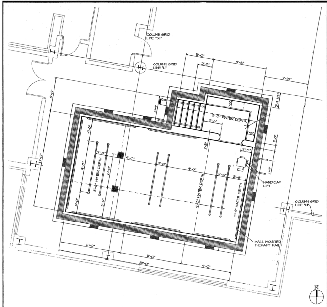
THERAPY POOL PLAN PL1.30-1 POOL RESURFACING – RIVERPLEX RECREATION & WELLNESS CENTER SCALE: 1/4"=1'-0"
